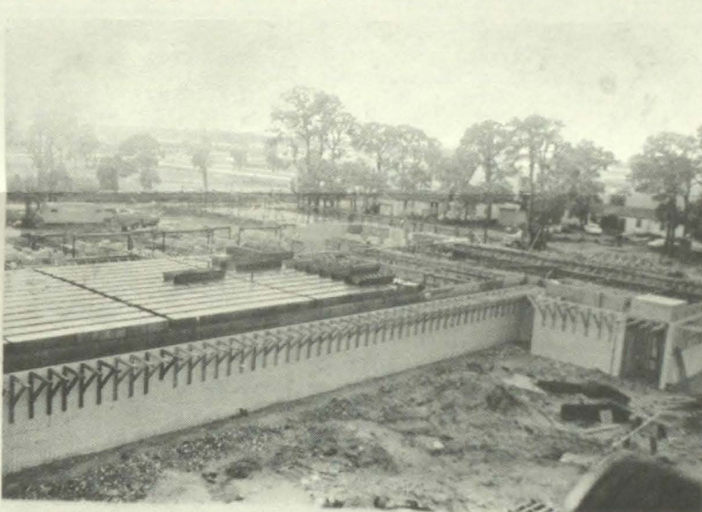
Most of the brick walls in Hamilton Court have been completed, and roofing material is being laid
